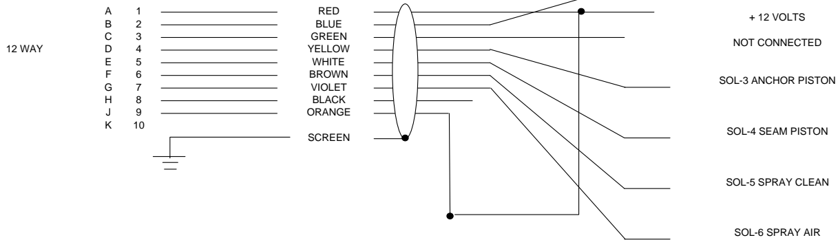
PCC2300 - SOLENOIDS CABLE ASSEMBLY
